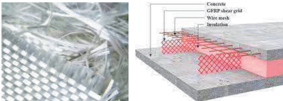
Figure 15. Glass Fiber Reinforced Polyester (GFRP) and Glass Fiber Reinforced Concrete (GFRC)
